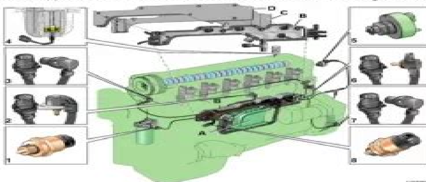
Figure 2 D12C, Engine sensors (some have dual functions)
