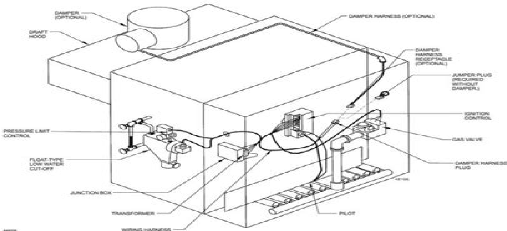
Figure 8 EGH steam boilers with float-type low water cut-off
