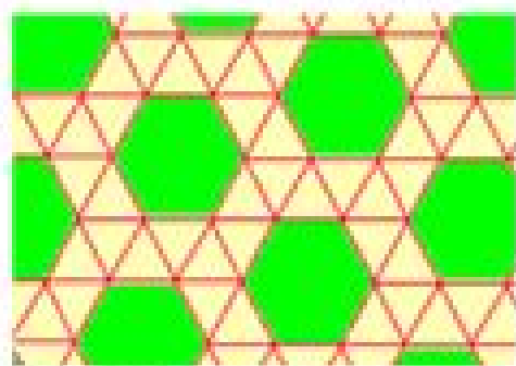
3.3.3.3.6
