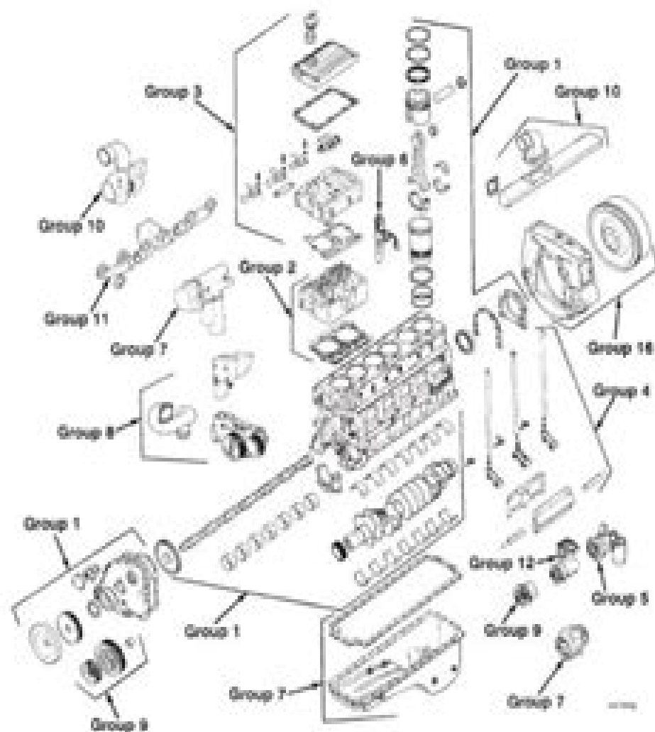
Cummins 23-Group System Exploded Diagram
