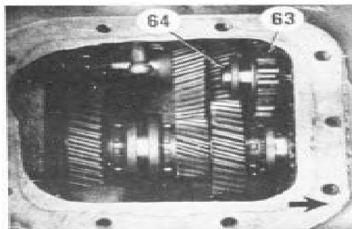
Fig. AC95—Model CA reverse idler gear (63) and shaft (64) installation view as seen through transmission cover opening.
